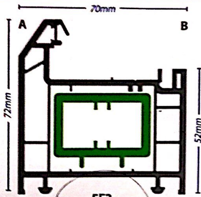
5F2 Large Outer Frame
