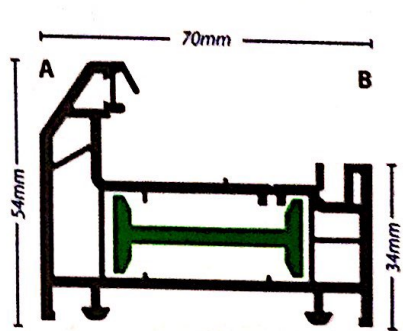
5F1 Slim Outer Frame
