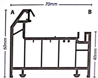
5F5 Intermediate Multi-chambered Outer Frame
