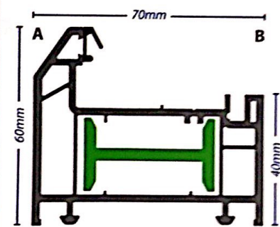
5F3 Intermediate Outer Frame
