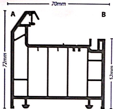
5F6 Large Multi-chambered Outer Frame
